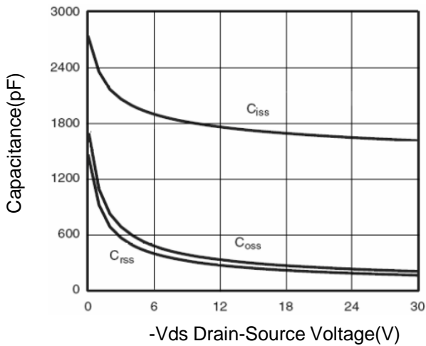
Figure 5. Capacitance
